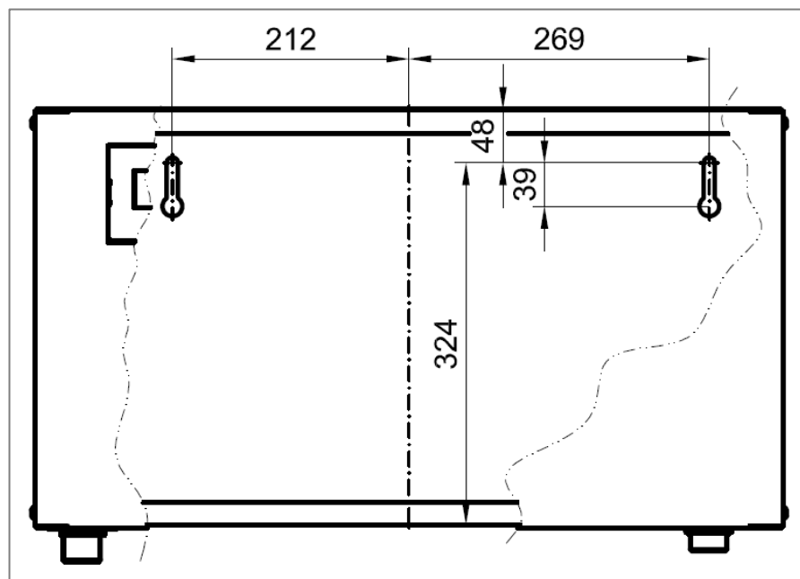
Figure 3: Drilling template compact domestic water heater
