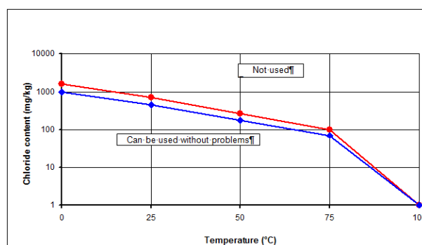
Figure 7 : Permissible chloride content depending on temperature
