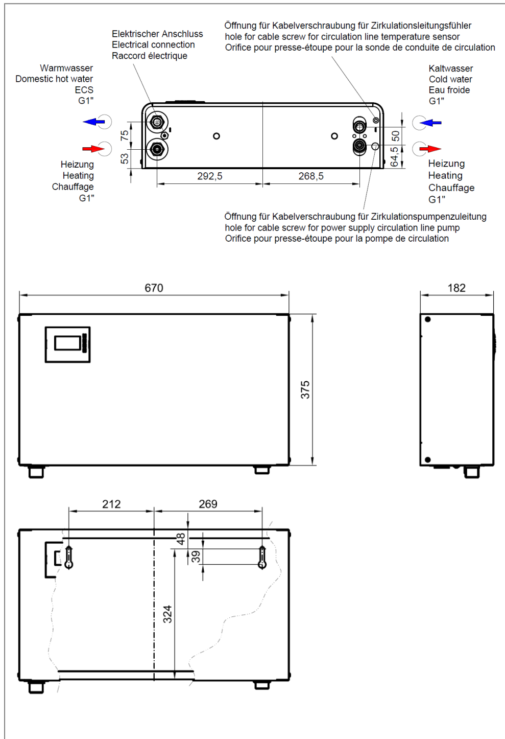
Figure 5: Connection dimensions in mm
