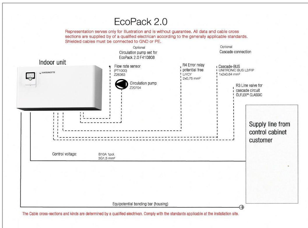
Figure 6: Cable list – EcoPack 2.0
