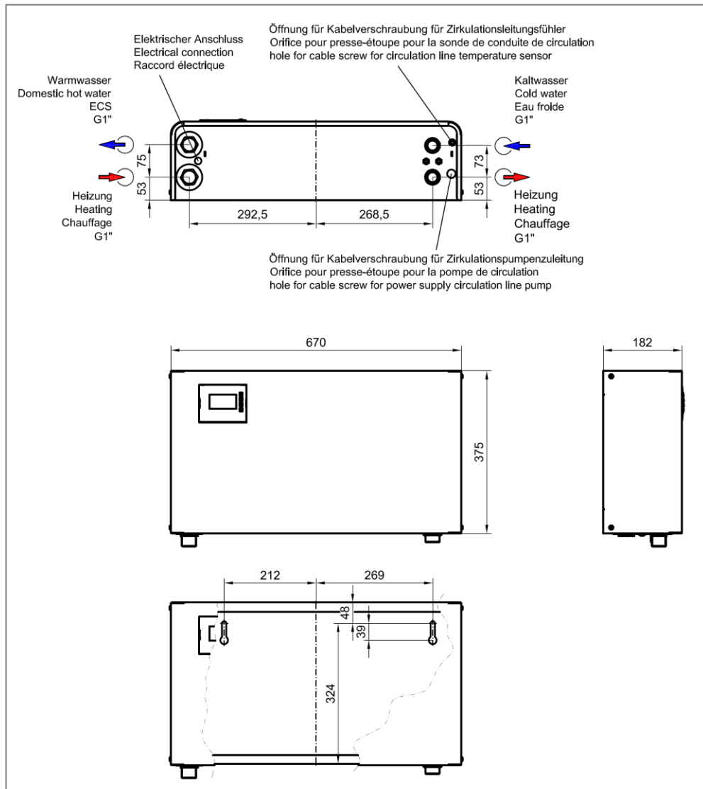
Figure 4: Connection dimensions in mm
