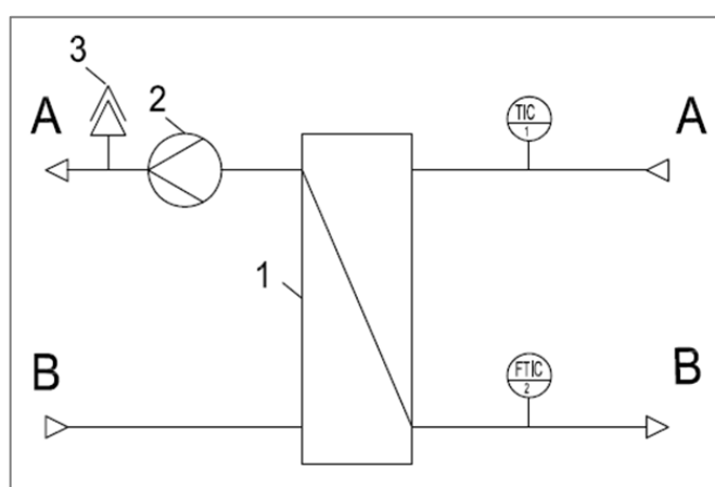
Figure 1: Electronic compact domestic water heater
